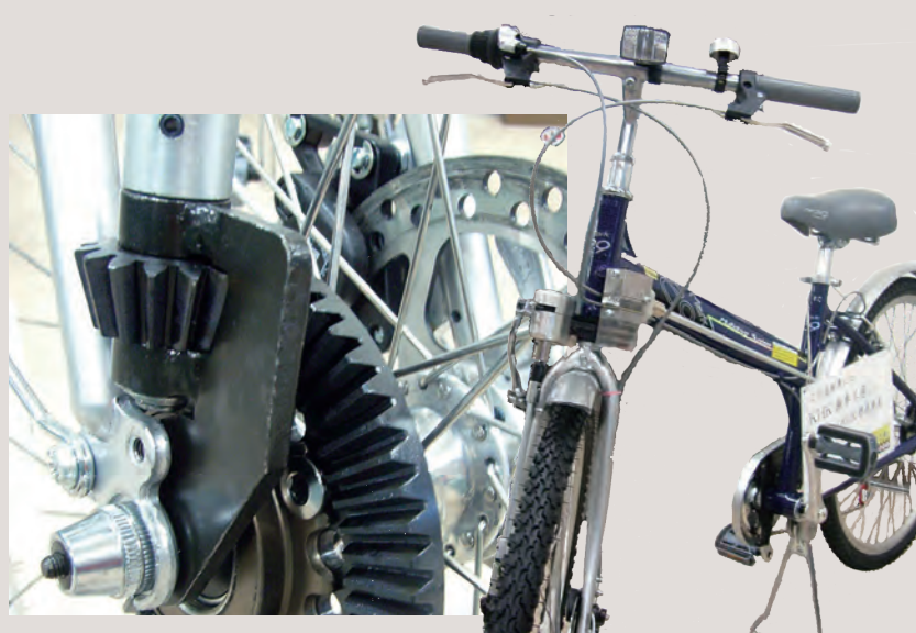
SB Bevel Gears are used in the driving components in both the front and rear wheels
