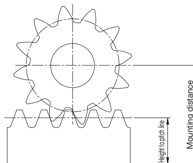
Mounting distance of a profile shifted gear and the meshing rack
