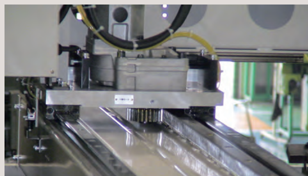
KRG Ground Rack used as a workpiece conveying device
