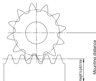
Mounting distance of profile helix gear and meshing rack
